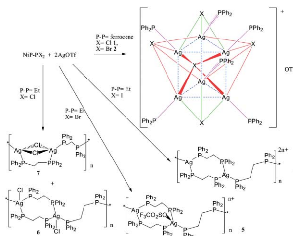
Scheme 1 A schematic representation of the products formed from the ligand migration reaction from \text{NiX}_2(\text{P-P}) ( \text{P-P} = \text{dppf}, \text{dppe} ) to \text{AgOTf} .
