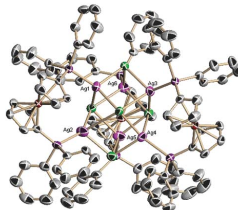
Fig. 1 ORTEP diagram of 1 , showing the cation. (Probability level of thermal ellipsoid 50%.)
